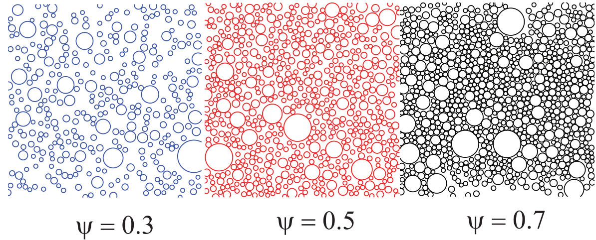
Sparse Packing, Shear Dominated Drift
