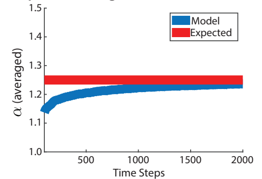
Crowding, Diffusive Drift
