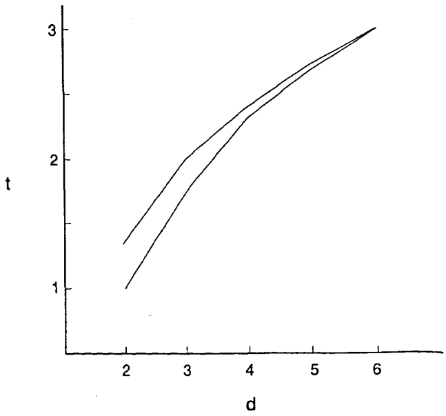
Figure 1. Proposed upper and lower bounds on the conductivity exponent t in terms of the percolation exponents \nu and \zeta . Numerical values for \nu and \zeta are used to evaluate the bounds in dimensions d = 2, 3, 4, 5 , and 6 . Straight lines have been drawn between these points.
