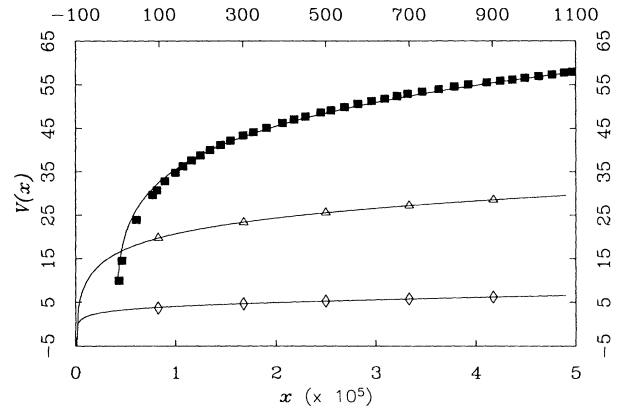
FIG. 1. The single-particle potential V(x) . The discrete points are from Ref. [11], obtained from numerical solutions of either a microscopic tight binding Anderson Hamiltonian with random site energies, or from a network of disordered quantum wires, for various values of disorder. The disorder is weakest for the squares, and strongest for the diamonds. The solid lines are from the potential (5) in the text, for \beta=2.30, 9.04 , and 27.07 chosen to fit the squares, triangles, and diamonds, respectively. The general agreement shows that the model defined by (5) describes a qualitatively appropriate phenomenological model for disordered conductors, with \beta increasing with increasing disorder.
