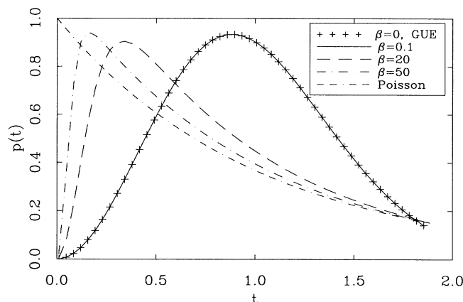
FIG. 2. The spacing distribution p(t) as a function of the spacing t between nearest eigenvalues for various values of the parameter \beta . For comparison, the universal GUE distribution, which coincides with the \beta=0 curve, and the Poisson (exponential) distribution are also included.
