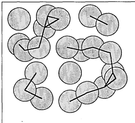
FIG. 9. Problem of random sites (overlapping discs).
