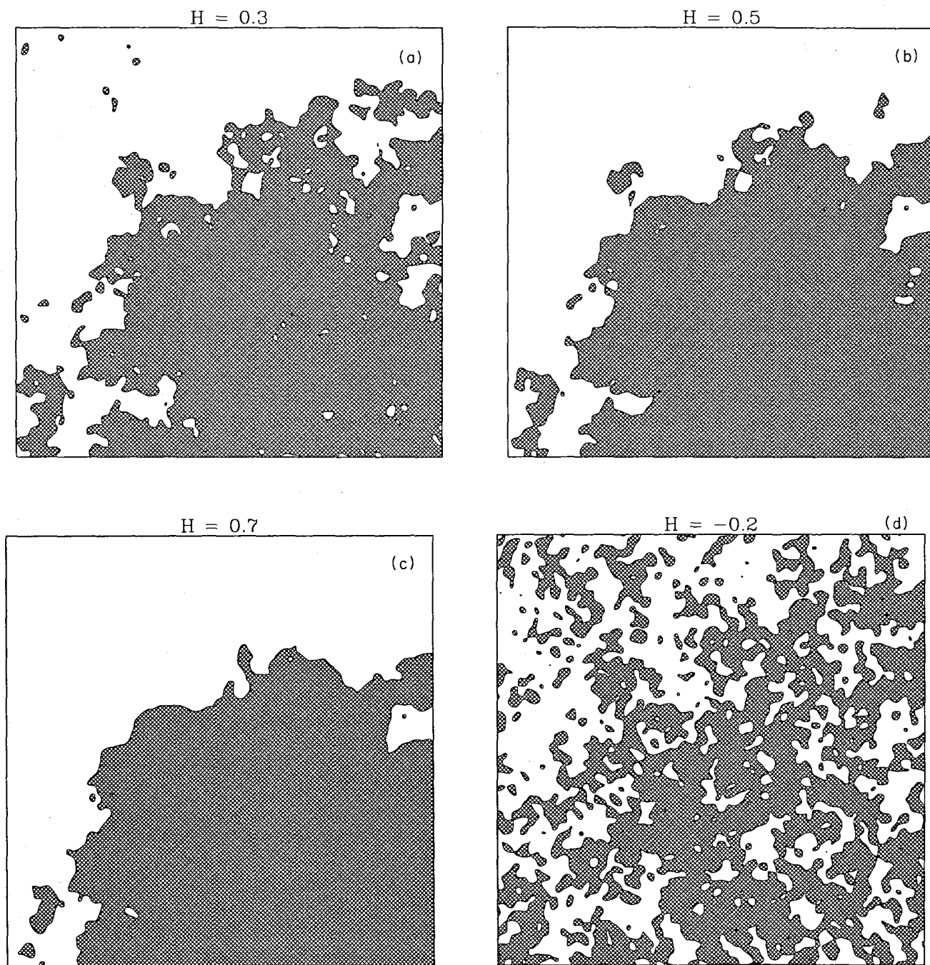
FIG. 14. Zero-level contour lines of the surfaces shown in Fig. 13.
