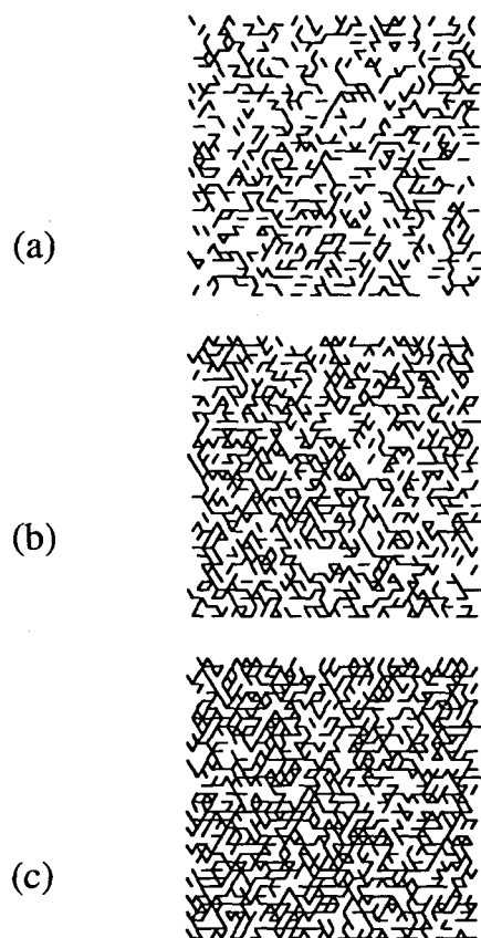
FIG. 4. Bond percolation clusters on a 2D triangular lattice at p = 0.25 (a), p = 0.3473 = p_c (b), and p = 0.45 (c).
