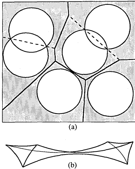
FIG. 8. The "Swiss-cheese" model. (a) The problem of circular voids in a background 2D transport medium. The sites of the equivalent lattice lie in the vertices of the Voronoi polyhedra (the sets of points from which a given void center is the closest one). The edges of the polyhedra represent bonds (solid lines). (b) A "neck" lying between three spherical voids.
