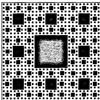
FIG. 1. Sierpinski carpet produced by removing from a square its central part with the size one-third the square edge. Then the procedure is repeated with each of the eight remaining parts, and so on ad infinitum . At the n th step of the procedure, it takes N_n = 8^n squares of the size \lambda_n = 3^{-n} to cover the remaining set, leading to the fractal dimension D = -\log N_n / \log \lambda_n = \log_3 8 .
