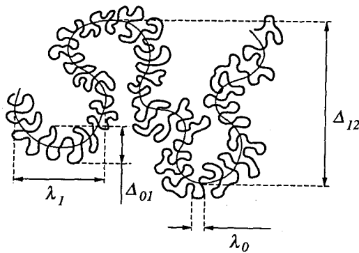
FIG. 19. Interaction of scales in terms of the behavior of a percolating isoline of the separated-scale potential (3.63).
