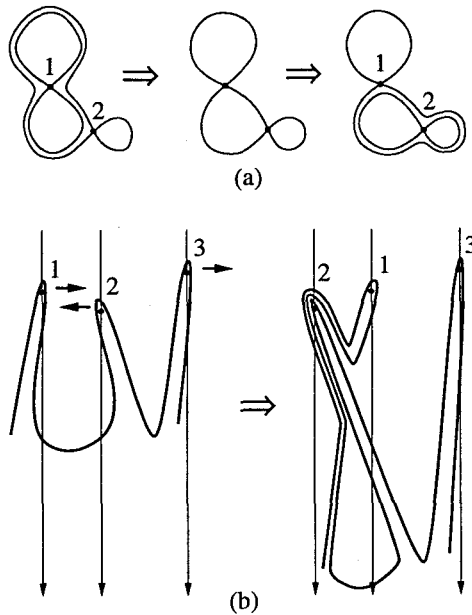
FIG. 28. Reconnection of two separatrices in a random flow. Reconnection takes place when two saddles, 1 and 2, cross the same level of the stream function (a). This is accompanied by the folding and stretching of a liquid curve (b). The light lines denote the separatrices, which are shown for simplicity to be straight and open (imagine a periodic boundary condition along the vertical direction). The curve drapes over the slowly moving saddle points 1, 2, and 3 and is rapidly stretched into the channels between the separatrices. The exponential behavior results from the intersection of separatrices, causing multiple foldings of the curve.
