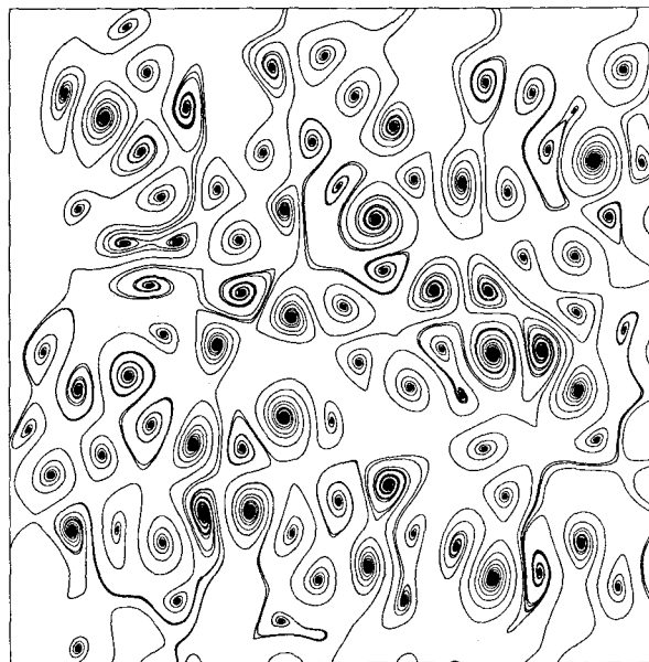
FIG. 30. Streamlines of weakly compressible flow (4.70) with \varepsilon = 0.1 and \psi(x, y) the same as in Fig. 10.
