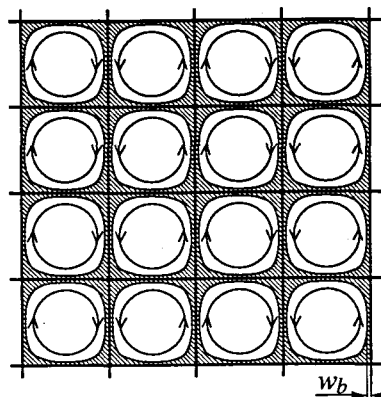
FIG. 20. Periodic system of convection rolls described by the stream function (4.26). The hatched region denotes diffusive boundary layers near the separatrices, where the tracer density gradients are localized in the high-Péclet-number limit.
