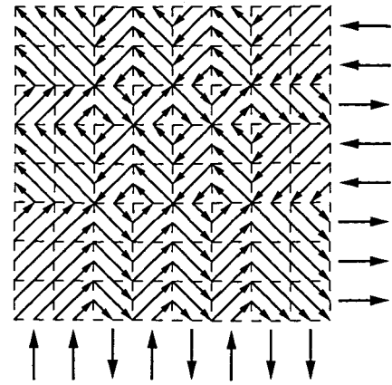
FIG. 32. Isotropic random flow of the “Manhattan-grid” type shown by the superposition of two mutually perpendicular random shear flows.
