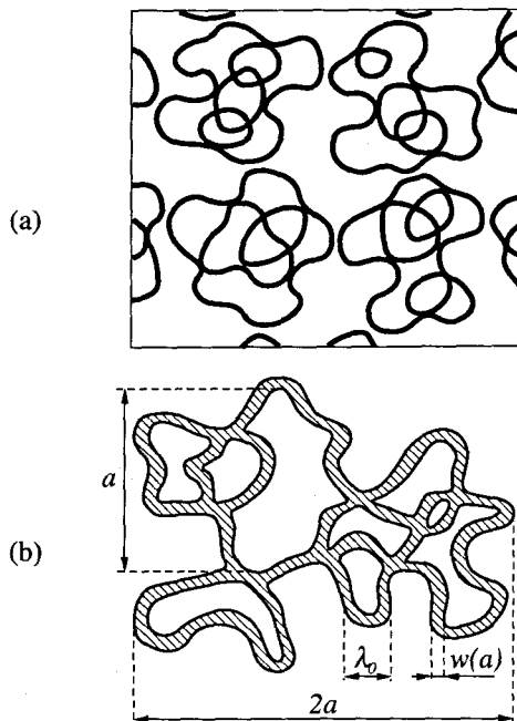
FIG. 17. Selecting contours by size. (a) The set of contours with linear size between a and 2a , consisting of a cells; (b) schematic of a typical a cell.
