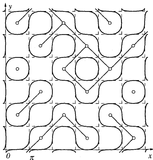
FIG. 11. Level lines \psi(x, y) = h of the potential \psi(x, y) = \sin x \sin y + \epsilon \psi_1(x, y) , \epsilon \ll 1 , |h| \leq \epsilon , where \psi_1 takes on independent random values with zero mean and unit variance in the unperturbed saddle points (where \sin x \sin y = 0 ). The contours of this potential represent the external and internal hulls of bond percolation clusters [ p(h) = 1/2 + h/\epsilon ] on a 2D square lattice with the sites \{(x, y): \sin x \sin y = -1\} . At h = 0 there exists an infinite contour corresponding to the external hull of the critical infinite cluster [ p(0) = \frac{1}{2} = p_c ].
