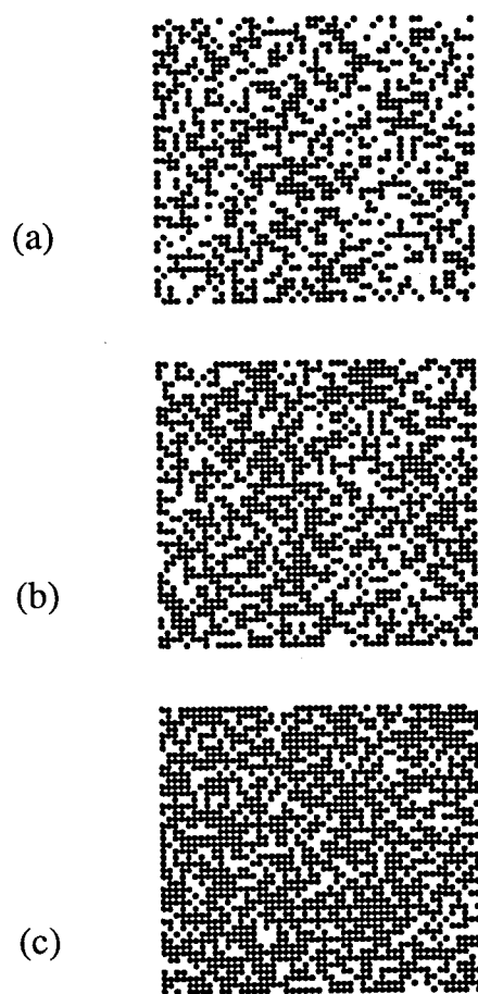
FIG. 3. Site percolation clusters on a 2D square lattice at p = 0.45 (a), p = 0.5927 = p_c (b), and p = 0.7 (c).
