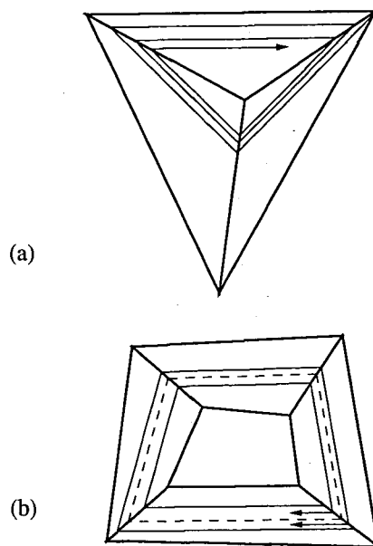
FIG. 37. Electric current streamlines in a strongly anisotropic polycrystal. These streamlines terminate in two types of traps: a focus (a) and a limit cycle (b).
