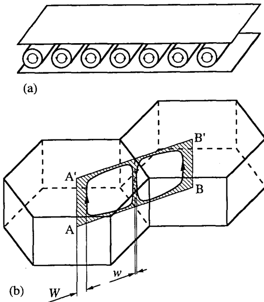
FIG. 21. Two types of steady Rayleigh-Bénard convection patterns: rolls (a) and hexagons (b). Axes AA' and BB' of the hexagons act on the streamlines as "free-slip" rigid boundaries. The hatched region shows the cross section of a diffusive boundary layer by the plane AA'BB' . To leave the trap of these two hexagons, a tracer particle has to diffuse (radially or azimuthally) all the way across the wider (near-axis) boundary layer ( W ).
