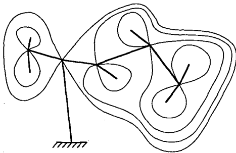
FIG. 34. Diffusion tree (branches shown in heavy lines) corresponding to passive transport in a topologically complex flow. For a nondegenerate flow each separatrix divides the plane into two inner regions and one outer region; hence all branching points on the tree are Y points.
