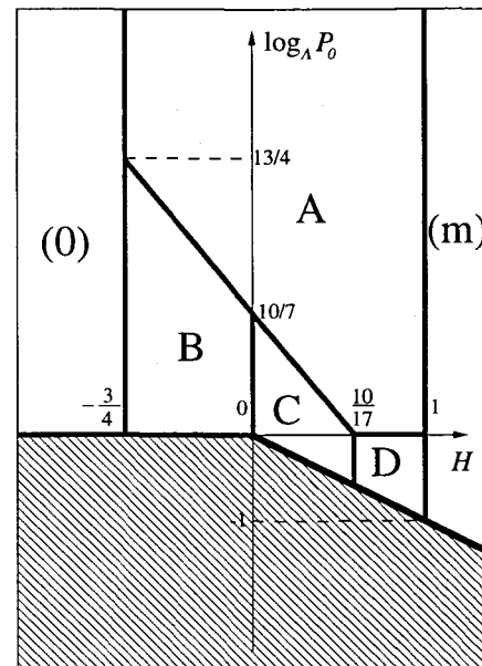
FIG. 23. Regimes of effective diffusion in a multiscale, steady, random 2D flow (Isichenko and Kalda, 1991c) shown in the parameter space ( H, \log P_0 / \log \Lambda ), where P_0 = \psi_{\lambda_0}/D_0 is the short-scale Péclet number and \Lambda = \lambda_m/\lambda_0 is the width of the flow spectrum. Expression D^* \simeq \psi_0 P_0^\alpha \Lambda^\gamma for effective diffusivity includes the following exponents in regimes (A–D): (A) \alpha = -1/(vd_h+2) , \gamma = (\nu H d_h + D_h)/(vd_h+2) ; (B) \alpha = H/(D_h - 2H) , \gamma = 0 ; (C) \alpha = 0 , \gamma = H ; (D) \alpha = (2 - D_h/H)/(vd_h+2) , \gamma = (\nu H d_h + D_h)/(vd_h+2) . Regimes (0) and (m) correspond to diffusion in the monoscale flows \psi_{\lambda_0}(x) and \psi_{\lambda_m}(x) , respectively. In the hatched region, D^* is of the order of D_0 .
