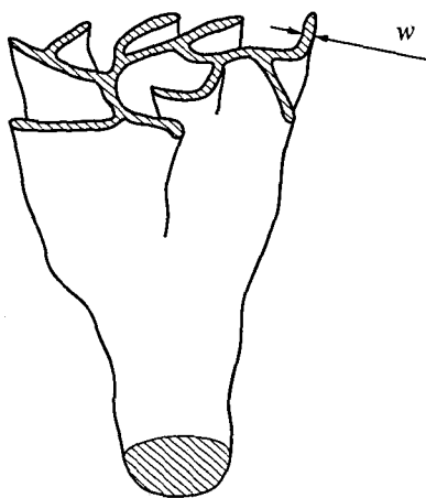
FIG. 39. Magnetic-flux tube in a magnetic field with a 3D random component. The tube is convoluted due to the exponentiation of neighboring magnetic lines. Because of the magnetic-flux conservation within the tube, the exponentiation of the lines leads to exponentially decreasing thickness w of the flux tube wall.
