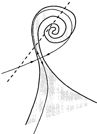
FIG. 26. Interaction of a liquid curve with a saddle point of a velocity field. Featured is the hooking of the curve over the saddle. The dashed line denotes the initial position of the curve, the heavy solid line is its final state, and the light lines with arrows show the velocity field.
