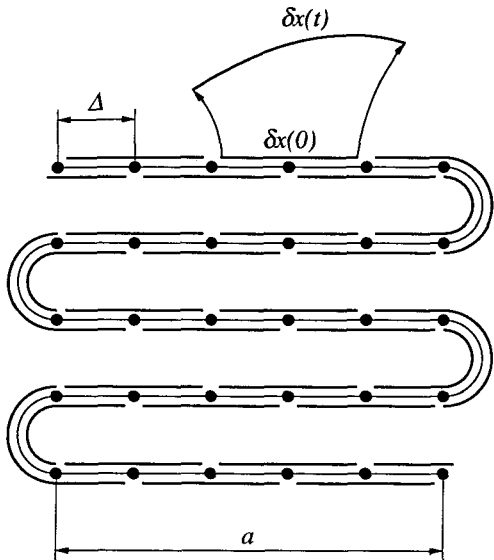
FIG. 25. Relation between the Kolmogorov entropy and the elongation of a liquid curve.
