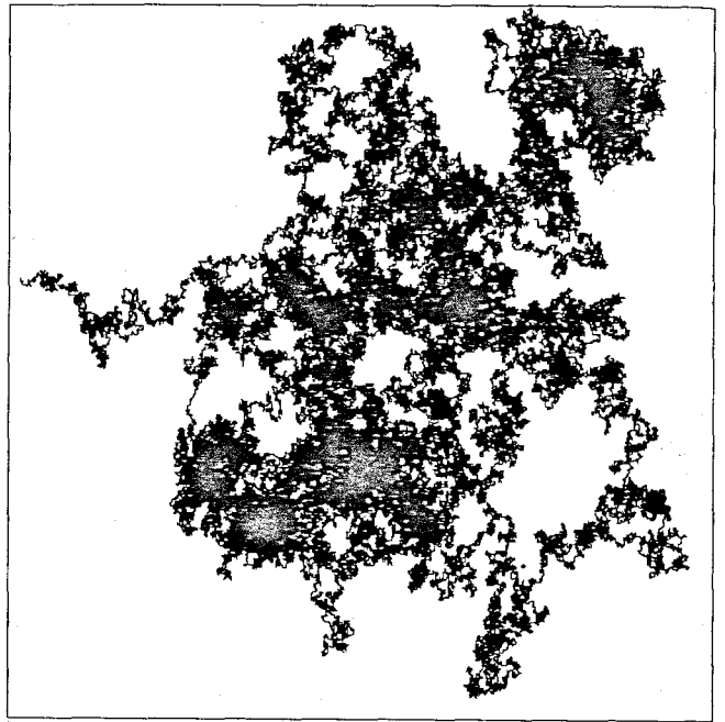
FIG. 2. Computer-generated trail of a Brownian particle. At any resolution of the trajectory, it asymptotically covers a finite area on the plane, because the fractal dimension D=2 .
