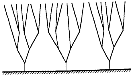
FIG. 35. Diffusion comb of a random flow, which looks like a thicket. The subdiffusive propagation along the "ground" (network of mixing convection cells) stems from the delay caused by random walk in the "bushes."
