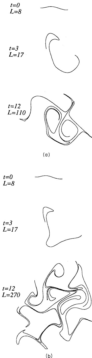
FIG. 24. Principal morphology of an incompressible map. The liquid-curve convolution is of two types: whorls (a) and tendrils (b) (Berry et al. , 1979). Whorls are generated by velocity fields of unchanged topology and lead to elongation of a passively advected curve that is asymptotically linear with time. Tendrils are created by essentially time-dependent flows and lead to an exponential elongation of a liquid curve. For the simulation, a stream function was chosen of the kind shown in Fig 10, with N = 5 frozen (a) or traveling (b) waves.
