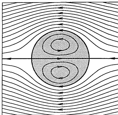
FIG. 22. Typical pattern of streamlines in a traveling dipole vortex, shown in the frame of reference moving together with the vortex. The hatched region surrounded by a separatrix (heavy line) represents the trapped fluid transported by the vortex.
