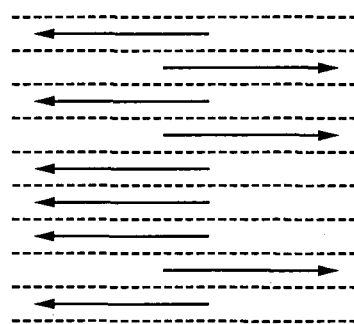
FIG. 31. Randomly directed shear flow with zero mean velocity but with a Brownian-type stream function.
