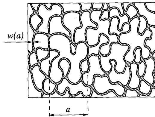
FIG. 16. Schematic of the set of contours with linear size larger than a : the a web.
