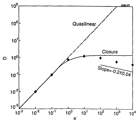
FIG. 29. Dependence of the turbulent diffusivity on the "Kubo number" K = v_0 / (\lambda_0 \omega) at \lambda_0 = v_0 = 1 (Ottaviani, 1992). The dashed line D \propto K represents the diffusion behavior in the high-frequency limit K < 1 and corresponds to the quasilinear scaling (4.64). The low-frequency behavior shows a systematic decline from the prediction of a Markovian closure theory (solid line; for a recent discussion see Fradkin, 1991).
