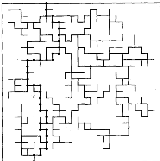
FIG. 6. Schematic of an infinite bond cluster on a 2D square lattice. The backbone is shown in heavy lines, the dangling ends in light lines. Markers denote a minimum path on the backbone.
