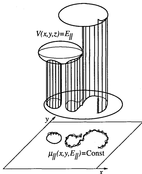
FIG. 41. Bounce motion of a magnetized electron, constrained to a cylinder of constant longitudinal invariant \mu_{\parallel} . The projection of the electron motion represents the averaged \mathbf{E} \times \mathbf{B} drift with a precession due to the dependence of this drift on z .
