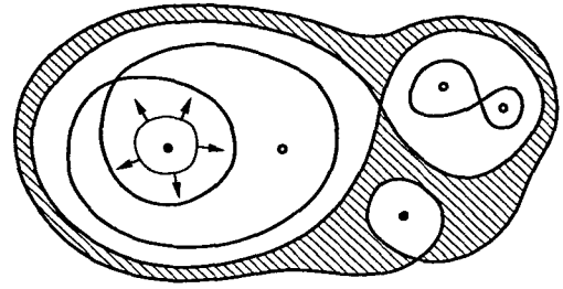
FIG. 15. Procedure of "contour dressing" (schematic). Separatrices (self-intersecting lines) come through saddle points. Extrema (maxima and minima) are shown by empty and solid circles, respectively. The hatched area lying between two neighboring separatrixes corresponds to the average area per saddle and is approximately constant ( \simeq \lambda_0^2 ) on each step of dressing.
