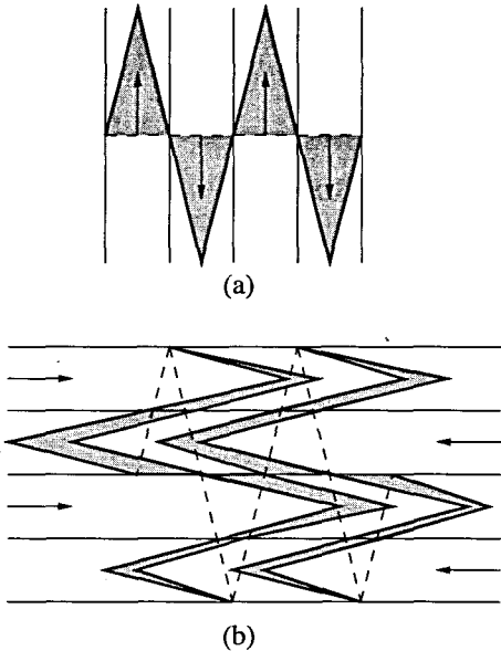
FIG. 27. Exponentiation of a liquid curve (the dashed line is the initial position and the solid heavy line is its final position) in a periodically changing shear flow during the first half-period (a) and during the second half-period (b).
