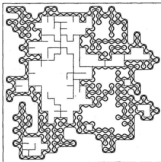
FIG. 7. Finite cluster (dashed lines), its external hull (heavy curve), and the unscreened perimeters (light curve).
