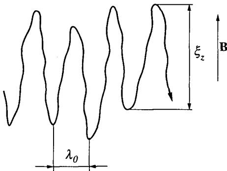
FIG. 40. Schematic of a current streamline corresponding to a steady flow of electric current across the magnetic field \mathbf{B} in a conducting medium with three-dimensional fluctuations.
