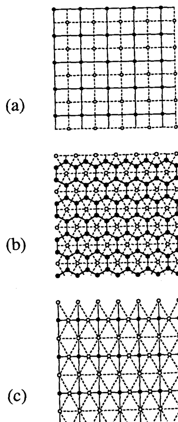
FIG. 5. Pairs of two-dimensional matching lattices, one shown by solid lines (for bonds) and filled circles (for sites) and the other by dashed lines and empty circles: (a) square-lattice bond problem is self-matching; (b) honeycomb and triangular lattices are bond matching; (c) square bonds match triangular sites.
