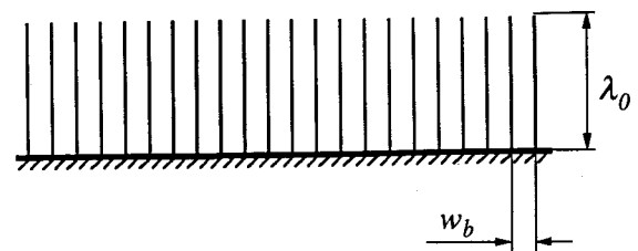
FIG. 33. Diffusion comb corresponding to a periodic array of convection rolls.
