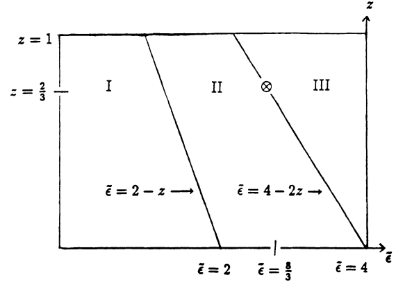
FIG. 1. The phase diagram for turbulent transport, for -\infty < \tilde{\epsilon} < 4 , 0 < z < 1 . Region I corresponds to Fickian scaling \nu(\tilde{\epsilon}, z) = 1 . In region II, we have \nu = (4 - \tilde{\epsilon} - z)/2 and in region III, \nu = 1 - \tilde{\epsilon}/4 . The Kolmogorov regime \tilde{\epsilon} = \frac{8}{3} , z = \frac{2}{3} is located on the boundary between the latter regions and is marked by \otimes .
