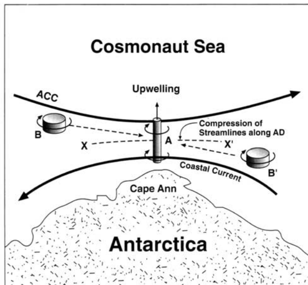
Figure 5. Mechanism for the Cosmonaut Polynya according to Comiso and Gordon [1996]. As water columns B (transported by the Antarctic Circumpolar Current (ACC)) and B' (transported by the Coastal Current) move both toward the polynya formation area A located over the Antarctic Divergence (AD), along XX' they must stretch in order to conserve absolute vorticity. Upwelling of warm deep water ensues. Reprinted from Comiso and Gordon [1996].
