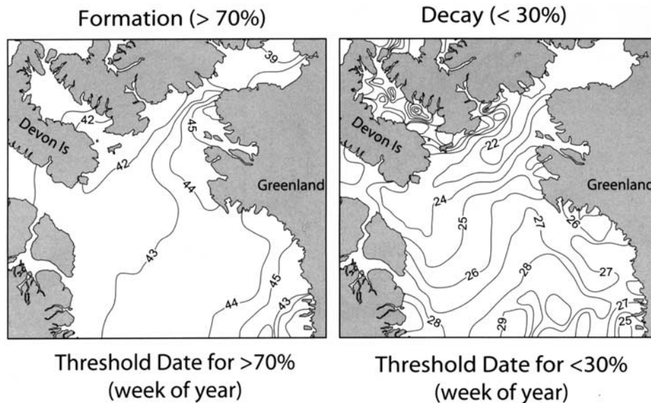
Figure 11. Average ice formation and decay in the North Water Polynya for 1979–1996. (left) Week of the year in which ice concentration becomes >70\% . (right) Week of the year in which ice concentration becomes <30\% . Note the late ice formation date along the western coast of Smith Sound (see Figure 1). Reprinted from Barber et al. [2001c] with kind permission of the Canadian Meteorological and Oceanographic Society.
