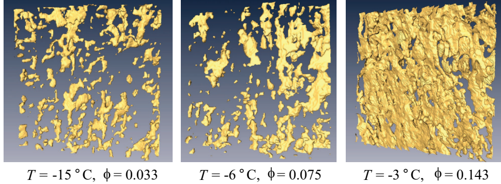
Figure 15: X-ray CT volume rendering of brine layers within a lab-grown sea-ice single crystal with S = 9.3 ppt. The (non-collocated) 8 \times 8 \times 2 mm sub-volumes illustrate a pronounced change in the micro-scale morphology and connectivity of the brine inclusions during warming.
