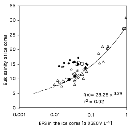
Fig. 4. Comparative relationships between bulk salinity and total EPS content (ice depth-averaged, in XGEQV L -1 ) for all ice-growth experiments. Starting solutions contained XG ( \Delta ), Colwellia EPS ( \bullet ), Melosira EPS (13-L tanks, \blacklozenge ; 200-L tanks, \circ ), or heat-treated (100 °C) Melosira EPS ( \diamond ). XG and Colwellia EPS had been exposed to 90 °C during preparation. The dashed portion of the functional line for XG ( n = 24 ) is an extension to the lowest observed bulk salinity for natural sea ice in this study.
