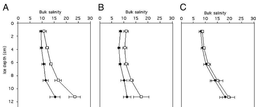
Fig. 3. Vertical profiles of bulk salinity of ice grown in 13-L tanks at -10^{\circ}\text{C} from saline solutions with (□) or without (●) Melosira EPS. The first experiment (A) was repeated by thawing the unsampled ice and refreezing the entire contents of the tank (B). For the third experiment (C), the contents were heated to 100^{\circ}\text{C} for 10 min before refreezing. Ice-growth rates were similar in A, B, and C ( 0.13\text{--}0.15 \text{ cm-h}^{-1} ). Error bars indicate SD of the mean ( n = 3 ).
