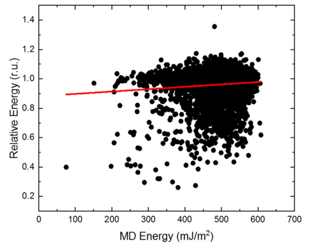
Fig. 11. Relative energies extracted from triple junction geometry of the as-deposited film for the 7304 boundary types examined in [36,37], plotted against the grain boundary energies calculated via MD in [36,37]. The least squares best fit line is plotted in red, with a correlation coefficient < 0.1 .
