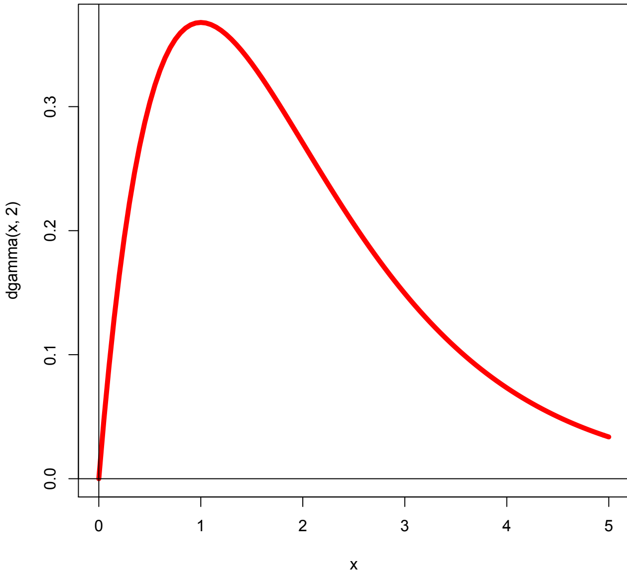
Density for Gamma, a=2, b=1
