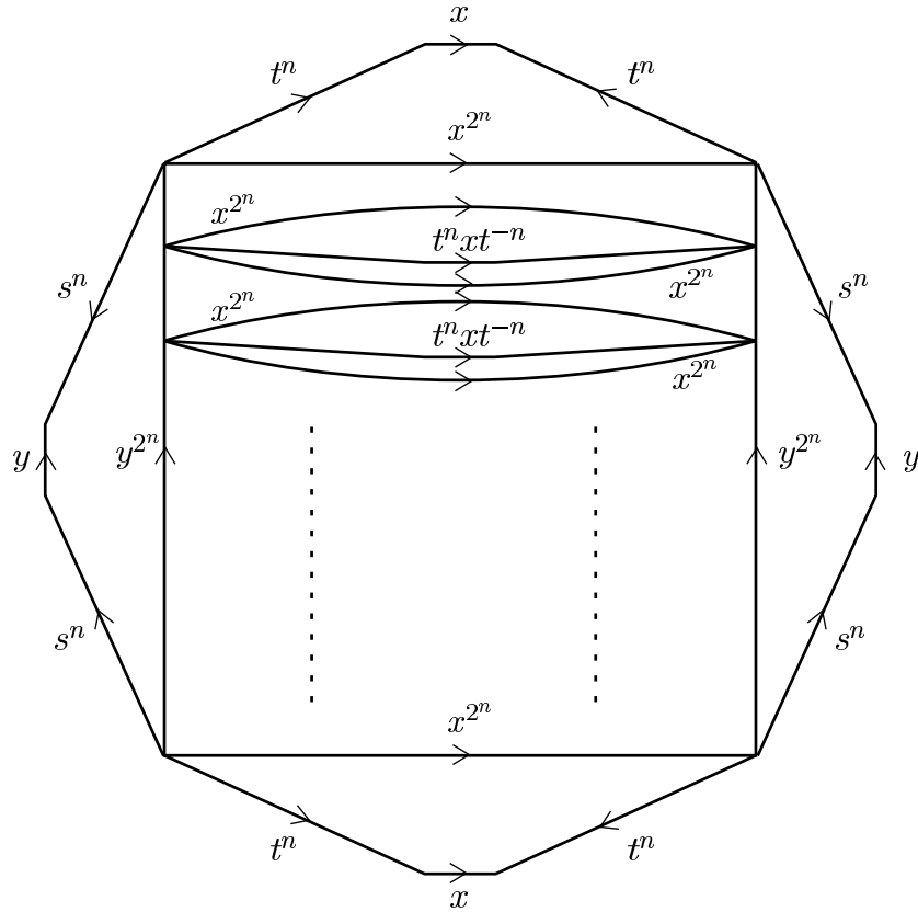
Figure 3: The diagram D'_n for w_n = [t^n x t^{-n}, s^n y s^{-n}] using shortcuts.
