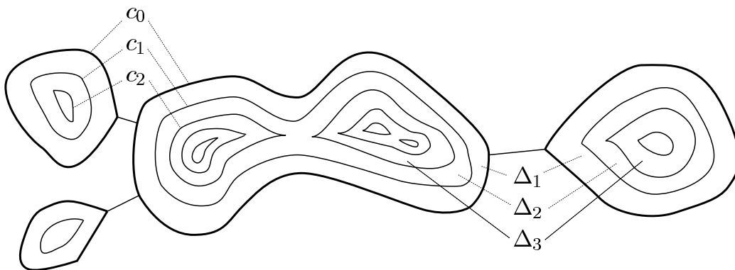
Figure 1: The annular decomposition of D .
