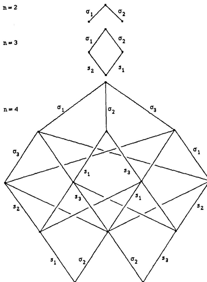
Fig. 1. Graph of the Bruhat order for Example 10.3 ( n = 2, 3, 4 ).
