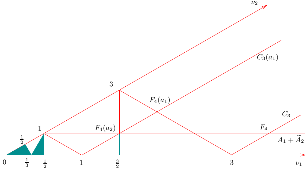
FIGURE 3. Spherical unitary dual attached to the orbit \tilde{A}_2
