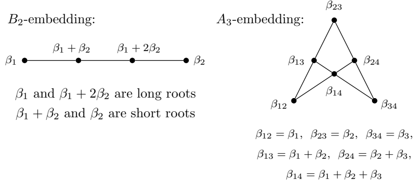
FIGURE 2. B_2 - and A_3 -embeddings
