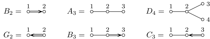
FIGURE 1. Dynkin diagrams of stellar root systems
