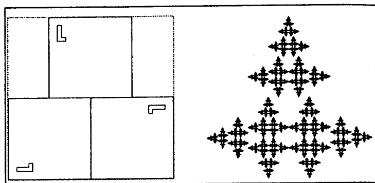
Figure 5.10 : Another IFS with three similarity transformations with scaling factor 1/2 .
