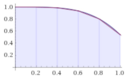
TRAP rule
