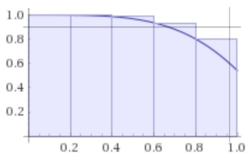
RECT rule
