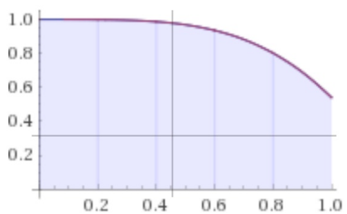
SIMP rule
