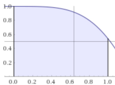
Integral Plot
