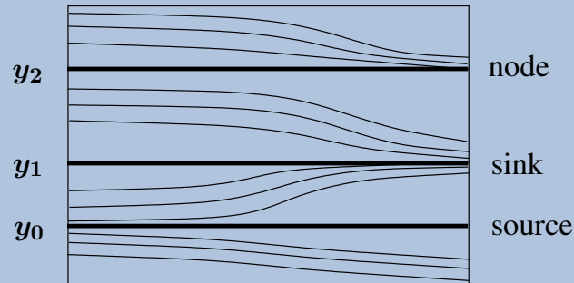
Figure 2. A phase diagram for an autonomous equation y' = f(y) . The graphic is drawn directly from phase line diagram Figure ??, using rules 1, 2, 3.
