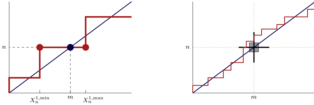
FIGURE 5.1. In both plots the diagonal line points in direction \xi(\lambda) . Left: the definition of X_n^{1,\min} and X_n^{1,\max} . Right: illustration of (5.1) and (5.4). The four arms of the cross centered at (m, n) = \lfloor N\xi \rfloor are of length rN^{2/3} each. The shaded box, also centered at (m, n) , has sides of length 2\delta N^{2/3} . For large r , the path has a high probability of entering and exiting through the cross and never touching the dotted lines. For small \delta , there is a positive probability, uniformly in N , that the path stays left of the top edge of the shaded box, completely avoiding the box.
