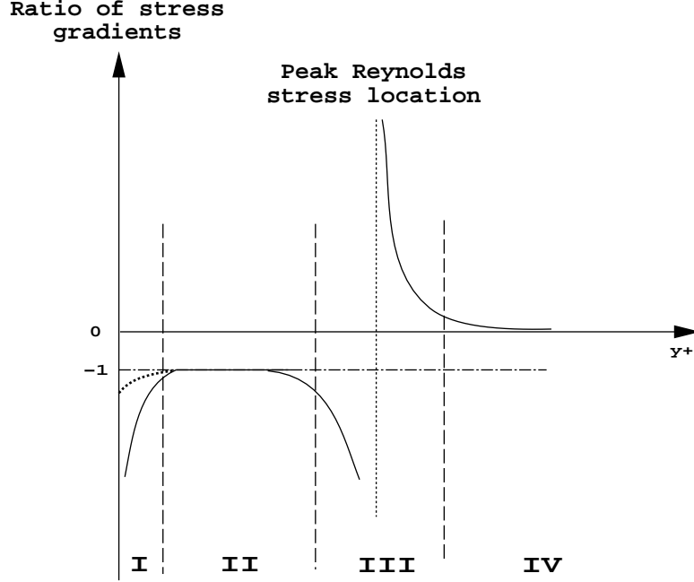
FIGURE 1. Sketch of the four layers of turbulent channel flow at a fixed Reynolds number; layer I is the inner viscous/pressure gradient balance layer, layer II is the stress gradient balance layer, layer III is the viscous/pressure gradient balance mesolayer and layer IV is the Reynolds stress/pressure gradient balance layer. Note layer I in the zero pressure gradient turbulent boundary layer is different from that of channel & pipe flow in that all of the terms in the boundary layer equation are zero at the wall.
