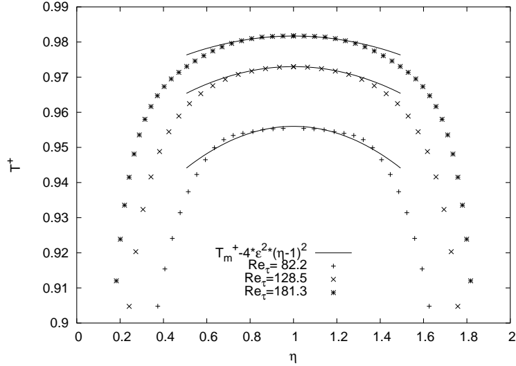
FIGURE 2. Reynolds stress around the peak, showing \frac{d^2 T}{d\eta^2} = O(\epsilon^2) and 1 - T_m = O(\epsilon^2) . Although these order of magnitude relations are clear, it is difficult to read off even the approximate value of \frac{d^2 T}{d\eta^2} . The case Re_\tau = 82 is from DNS of Bech et al. (1995), and the other two cases are from DNS of Kawamura, Abe & Shingai (2000)
