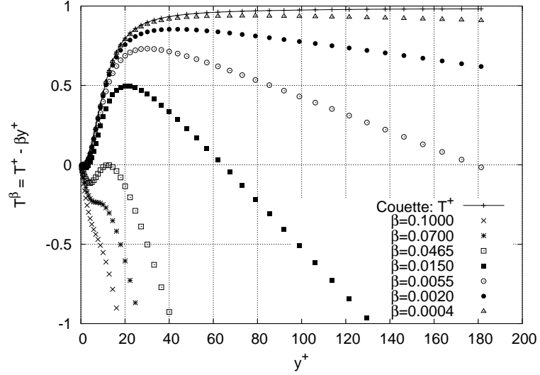
FIGURE 3. Adjusted Reynolds stress profile for various values of \beta . The case \beta = \epsilon^4 corresponds within O(\epsilon^2) to the genuine Reynolds stress for Couette flow (see Section 3.4.6), and \beta = \epsilon^2 is an approximation to that for pressure driven channel flow. The DNS data is from Kawamura, Abe & Shingai (2000), \delta^+ = Re_\tau = 181.3 and \epsilon = .074 .
