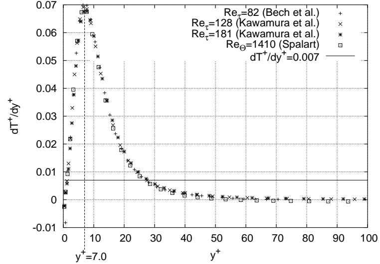
FIGURE 4. Inner normalized Reynolds stress gradient for a variety of flows. The turbulent Couette flow data are from Bech et al. (1995) and Kawamura et al. (2000). Also included are turbulent boundary layer DNS from Spalart (1988).
