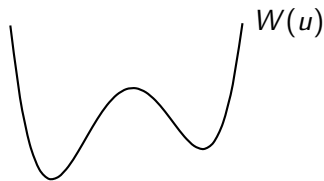
Figure: Plot of double well potential W(u) .
