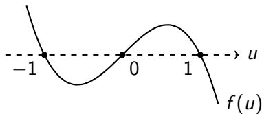
Figure: Plot of bistable nonlinearity f(u) = -W'(u) .
