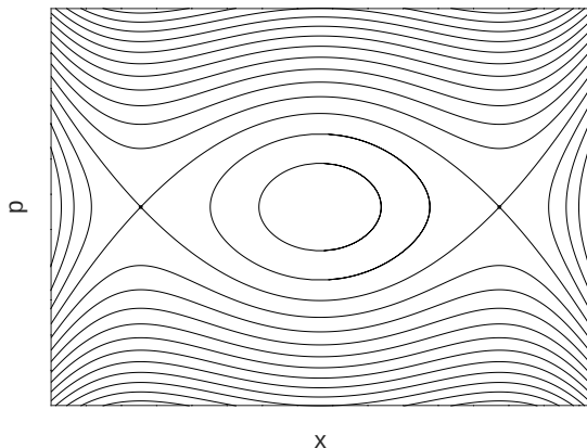
Figure: Contour plot for H(\dot{\xi}, \xi) = \frac{1}{2}\dot{\xi}^2 - W(\xi) .
