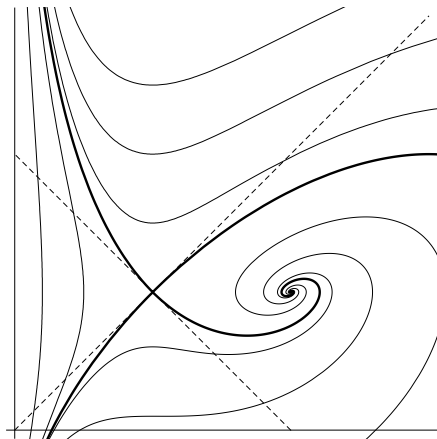
Figure: Global stable and unstable manifolds (in bold) of a hyperbolic fixed point for a planar nonlinear system. The linearized stable and unstable subspaces are drawn with dotted lines.
