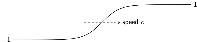
Figure: graph of u(x, t) at some fixed time.
