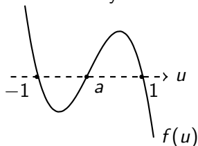
Figure: Plot of asymmetric bistable nonlinearity f(u) = -W'(u) .
