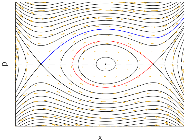
Figure: \Gamma_1(c) red and \Gamma_{-1}(c) in blue when c = 0 .
