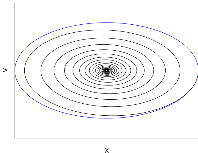
Figure: In blue the \frac{1}{4} level set of the energy H(v, x) = \frac{1}{2}v^2 + \frac{1}{4}x^2 . In black a solution of the damped mass-spring system started at (x_0, v_0) = (1, 0) .
