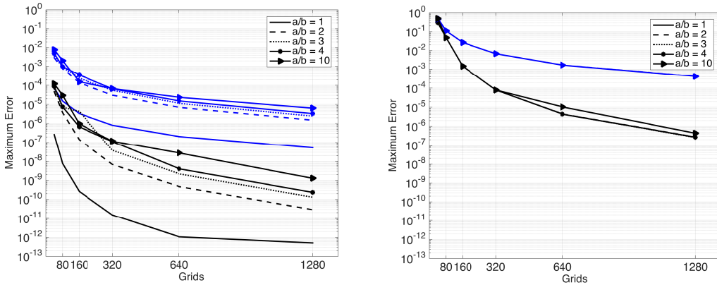
FIG. 6.4. Grid convergence using BDF2-DPM2 (blue) and BDF4-DPM4 (black) is compared for several different interfaces \Gamma: x^2/a^2 + y^2/b^2 = 1 with increasing aspect ratios a/b . The results are presented for the test problem (6.5), (6.9) with material coefficients \lambda_1 = \lambda_2 = 1 (left figure) and for the test problem (6.5), (6.10) with material coefficients \lambda_1 = \lambda_2 = 1 (right figure). Similar results are produced by DPM for the same test problems but with different material coefficients in different subdomains, as well as for error in the gradient of the solution.
