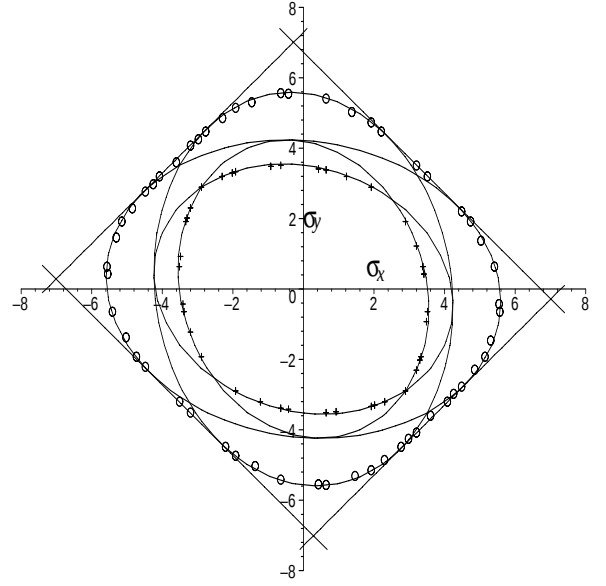
Fig. 7 Two-dimensional case; Region \mathcal{F}_1 lies inside of the region given by crosses, while region \mathcal{F}_2 lies outside of the region given by circles. The forbidden region \mathcal{F}_f lies between the regions.
