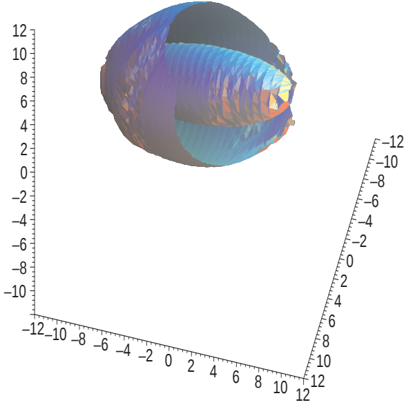
Fig. 1 Assembly of bounds: The interior region (intersection of ellipsoids) defines the bound of the set \mathcal{F}_1 (stress in the weak material), the outer region defines the zone \mathcal{F}_2 of optimality of the stress in the strong material, and the region between defines the forbidden region. One of the materials has zero Poisson ratio.
