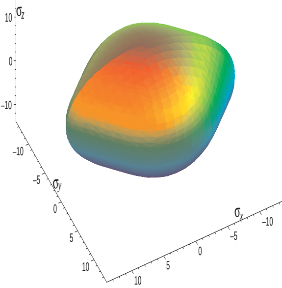
Fig. 5 The intersection of three ellipsoids defines the bound of the set \mathcal{F}_2 when one of the materials is void.
