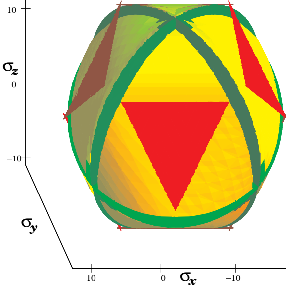
Fig. 4 The black triangular region is the third-rank laminate. White and gray regions show where the second and first-rank laminates are optimal, respectively.
