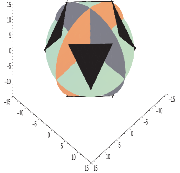
Fig. 8 One of the materials is void. The boundary of the permitted region of the strong material. Observe that the components of the boundary that correspond to optimality of simple laminates disappear.
