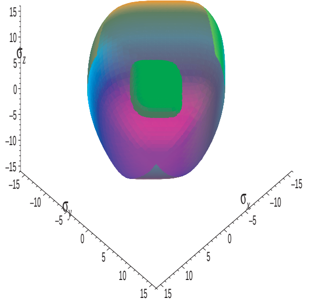
Fig. 3 The interior region of the small ellipsoid defines the bound of the set \mathcal{F}_1 , and the region between the ellipsoids defines the forbidden region when one of the materials has nonzero Poisson ratio.
