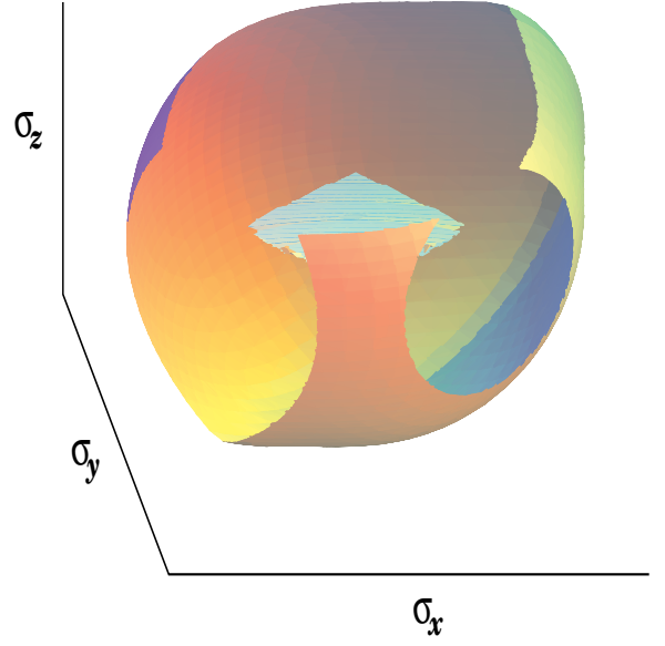
Fig. 6 The interior region of the small ellipsoid defines the bound of the set \mathcal{F}_1 , and the region between the ellipsoids defines the forbidden region when one of the materials is void.
