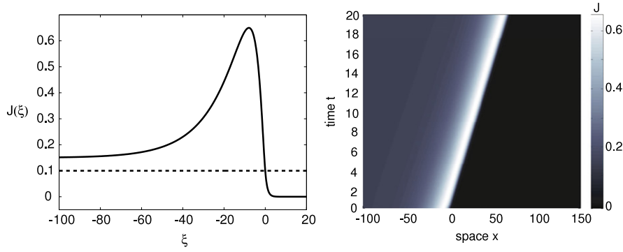
Fig. 2. (Left) Profile of analytical front solution J(\xi) = U(\xi) - A(\xi) for parameter values \theta = 0.1 , \alpha = 20 , \beta = 0.2 , \epsilon = 5 , and \gamma = 0.05 . Wavespeed c_+ is specified by Eq. (3.15). Note that, as \xi \rightarrow -\infty , J(\xi) \rightarrow 1/(1 + \alpha\beta) - \gamma . (Right) Corresponding space–time plot of a traveling front obtained by solving the system (2.1) numerically with the analytical front solution taken as the initial condition.
