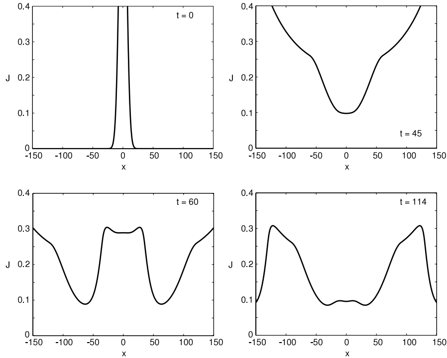
Fig. 14. Snapshots of total input current J(x, t) as a function of space x for times (Top left) t = 0 ; (Top right) t = 45 ; (Bottom left) t = 60 ; and (Bottom right) t = 114 . Oscillating core is centered at x = 0 and periodically emits pulses of activity after an initial traveling front.
