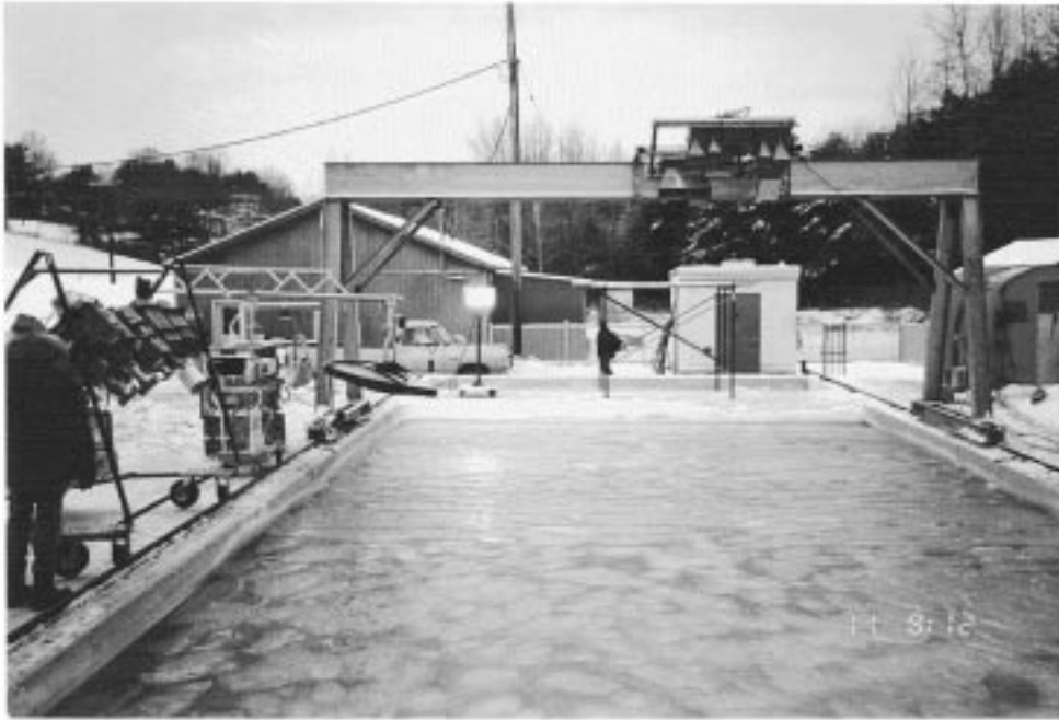
Fig. 3. The sea ice test facility constructed at the CRREL. Pictured is pancake ice, a type of ice that forms in the presence of a wave field. Observations were made from the sides of the pond and from a movable gantry. A removable, refrigerated roof was used to regulate surface conditions, including temperature and the amount of snowfall.
