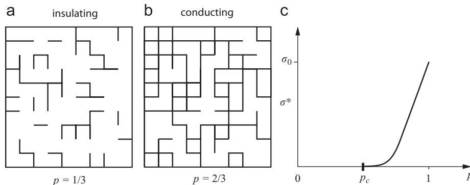
Fig. 2. The two-dimensional square bond lattice below its percolation threshold p_c=1/2 in (a), and above its threshold in (b). Below p_c , there is no bulk transport, and above p_c the transport coefficient takes off with power law behavior, as shown in (c).
